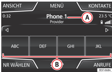
Abb. 20 Hauptmenü PHONE.
